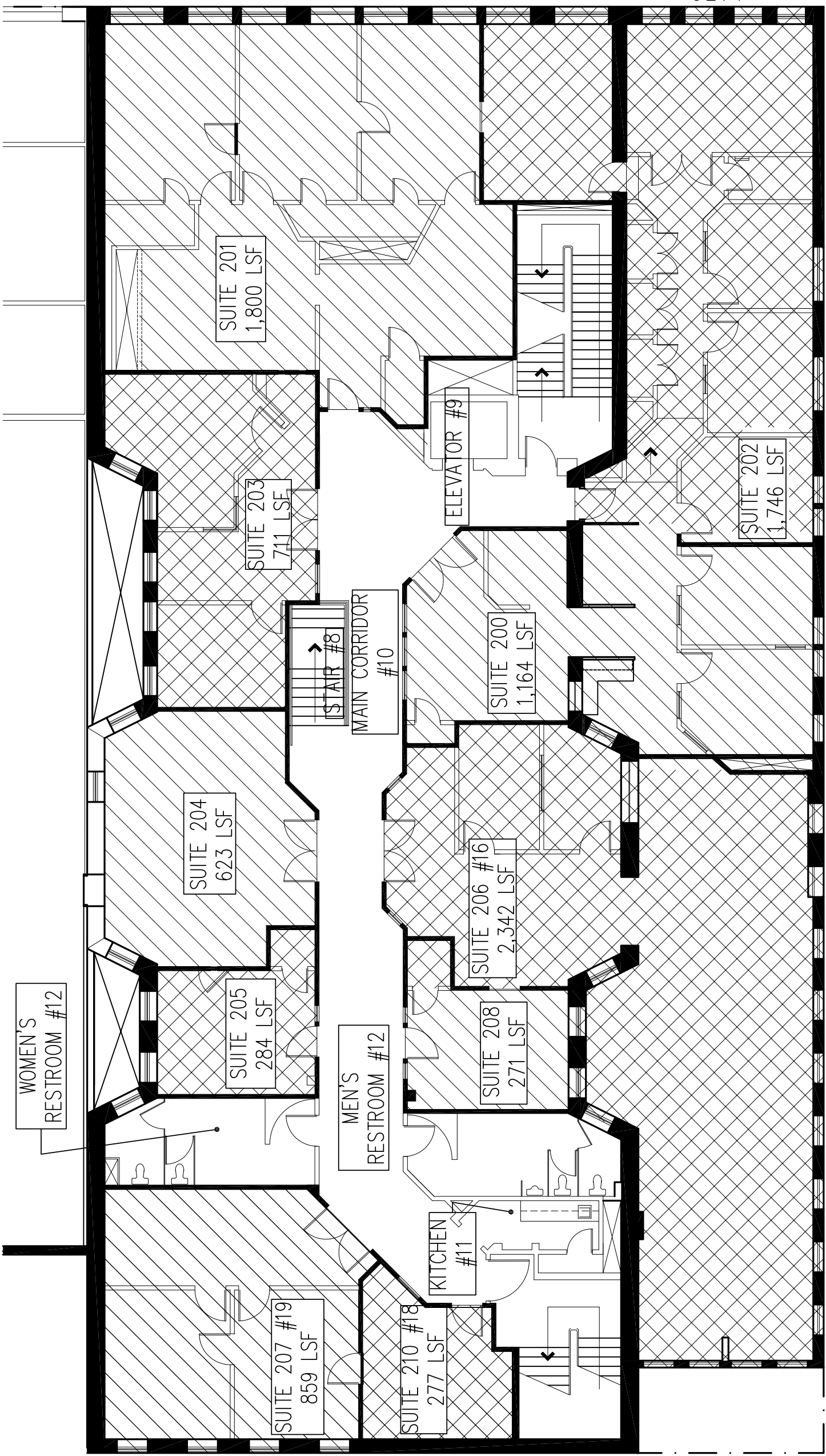
1 SECOND FLOOR PLAN A120 3/32" = 1'-0"
